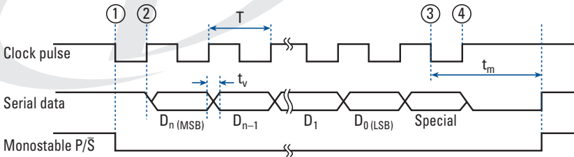
Figure 1 SSI Communication Format
